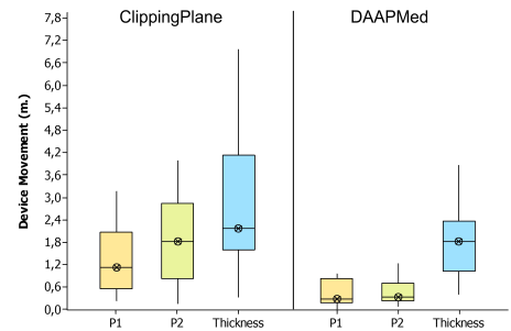
Figure 7: Input device footprints. The boxes show the interquartile range with the median as the horizontal bar. The whiskers extend to the minimum and maximum of the data. For point selection it is clear that DAAPMed method performed significantly better than CP.
