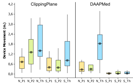
Figure 8: Input device footprints. The displacement carried out by the device is split in two states: navigation ( N_{\{P_1, P_2, Th\}} ) and selection ( S_{\{P_1, P_2, Th\}} ). The boxes show the interquartile range with the median as the horizontal bar. The whiskers extend to the minimum and maximum of the data.
