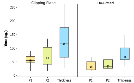
Figure 6: Results of the completion task timings. The boxes show the interquartile range with the median as the horizontal bar. The whiskers extend to the minimum and maximum of the data. CP exhibits longer selection times.
