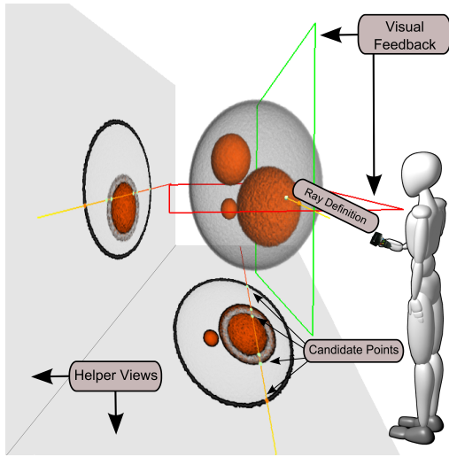
Figure 2: DAAPMed metaphor: A ray is used for selection, and a couple of supporting planes help the user to locate it in relation to the 3D structures. Potential anchor points, represented by colored small spheres, are computed as the intersections of the ray with the isosurfaces. Finally, Helper Views provide a better perception of the ray position as well as aids disoccluding interior candidate points. Notice that the bottom view shows that the large orange sphere is hollow.
