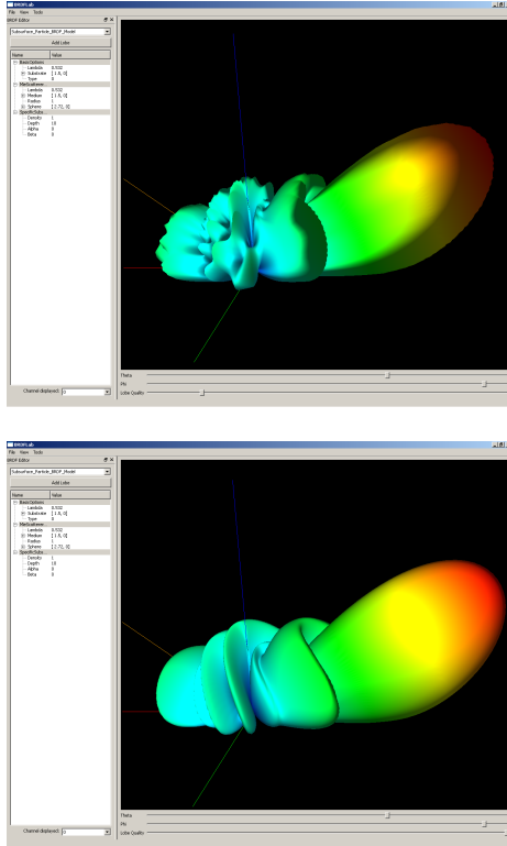
Figure 8: Simulation obtained with the Scatmech library using a subsurface particle model. Top using a 32x32 resolution texture and bottom 150x150.
