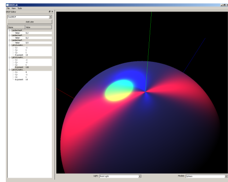
Figure 4: Point light rendering of a sphere. The BRDF uses a Fixed combination of a Lambertian lobe and an anisotropic Lafortune lobe, where each channel uses a different lobe. The flexibility of this representation is shown.
