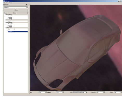
Figure 6: Real time rendering of a car model with filtered importance sampling environment mapping light.
