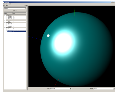
Figure 3: Point light rendering of a sphere. The BRDF uses a Linear combination of a Lambertian lobe and an isotropic Lafortune lobe, where all the channels share the same lobe.
