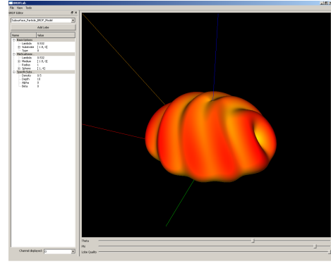
Figure 9: Simulation obtained with the Scatmech library using a subsurface particle model and a 150x150 resolution texture.
