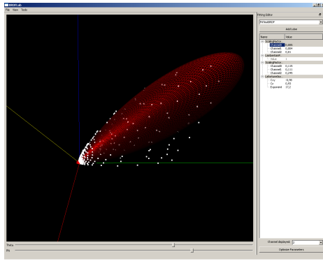
Figure 2: The blue metallic paint material of the MERL database is fitted to a linear combination of a Lambertian lobe and an isotropic Lafortune lobe.
