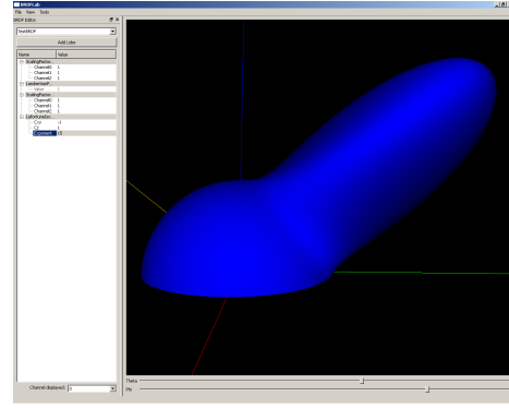
Figure 1: Linear combination of a Lambertian lobe and an isotropic Lafortune lobe. Our system allows to interactively modify the incoming direction and the parameters of the lobes to see how the shape looks like.
