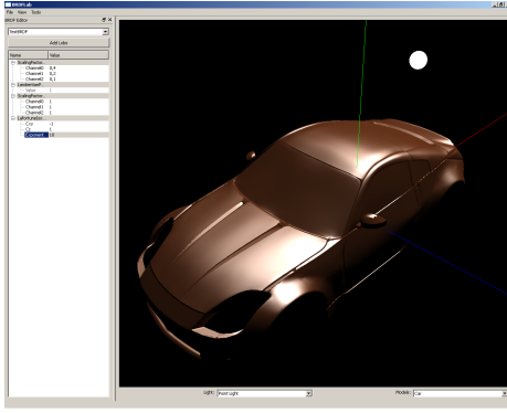
Figure 5: Point light rendering of a car model. The BRDF used is a Linear combination of a Lambertian lobe and an isotropic Lafortune lobe.
