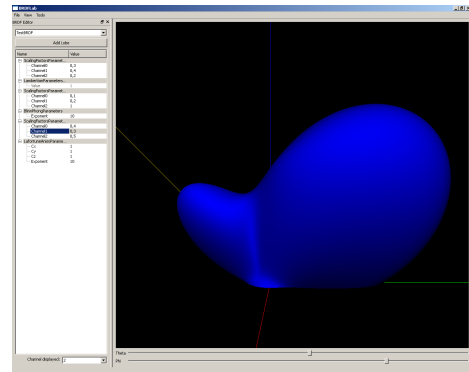
Figure 7: Linear combination of a Lambertian lobe, an anisotropic Lafortune lobe and a Blinn-Phong lobe.
