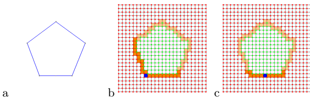
Figure 1: (a) The discretization of a pentagon defines a set of cells which can be used to compute cell to cell unconstrained visibility. (b) Visibility from a cell containing a vertex results in the cells stabbed by its two adjacent edges, while (c) visibility from a cell on an edge results only in the cells stabbed by that edge.
