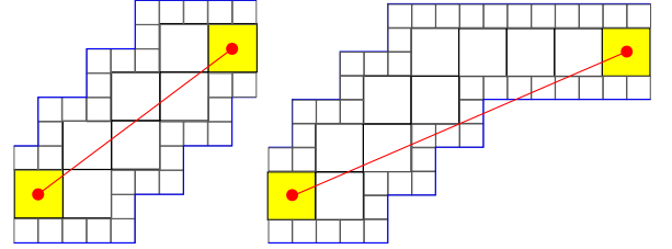
Figure 6: Visibility computation for the examples shown in Figure 4. Testing a segment that connects two cell's centers for intersection with the eroded object (shown in blue) is enough using the erosion based technique.
