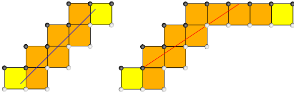
Figure 4: 2D examples of cell to cell visibility. In the picture on the left the two yellow cells see each other, while in the figure on the right they do not.
