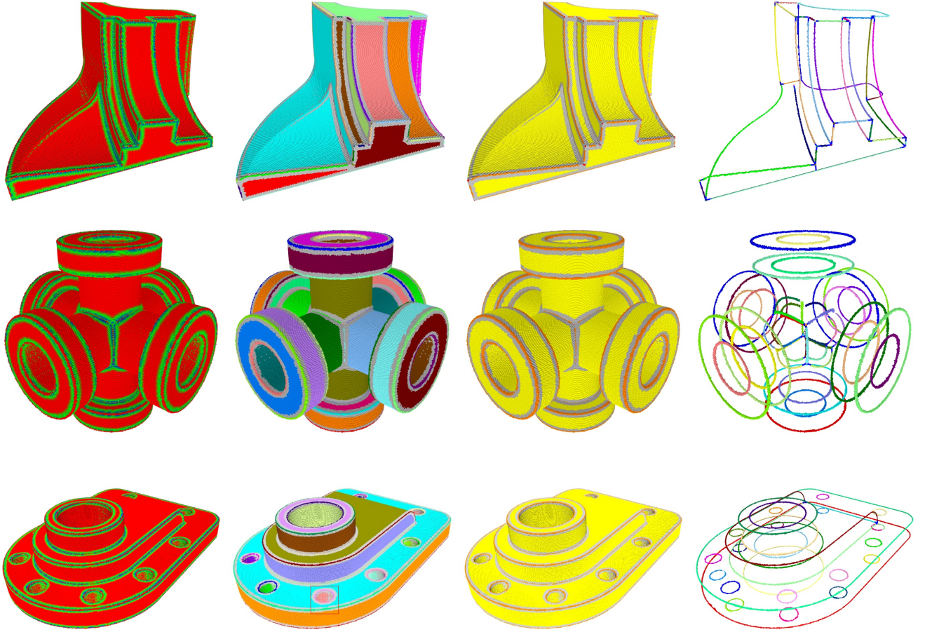
Figure 12: From left to right: visibility maps, identified components, their classification and the resulting connectivity graphs. From top to bottom: the models of the FANDISK, a CROSS pipe and another mechanical part (COVER).
