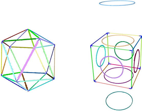
Figure 10: Resulting connectivity graphs of the icosahedron and the mechanical part models. Vertex components are represented as spheres. The 30 edges and 12 vertices of the icosahedron are successfully recovered, together with their correct connectivity.
