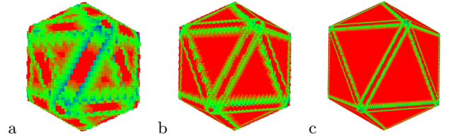
Figure 11: Components become easier to identify using larger resolutions when computing their visibility maps. The images show the visibility map of an icosahedron discretized at different resolutions: (a) 64 \times 64 \times 64 (b) 128 \times 128 \times 128 (c) 256 \times 256 \times 256
