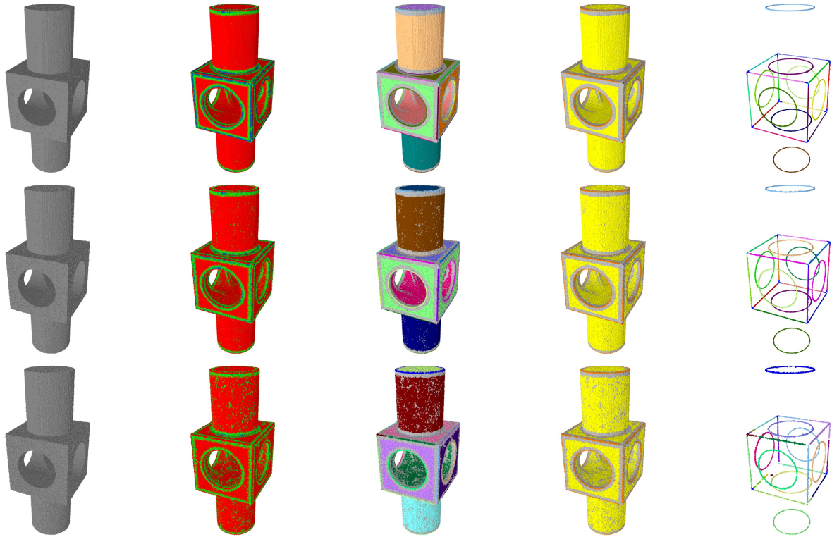
Figure 14: From left to right: binary grids, visibility maps, identified components, their classification and the resulting connectivity graphs. Top row shows the binary grid of a mechanical part corrupted with white gaussian noise of \sigma = 0.22 . Middle and bottom rows show the same model corrupted using a gaussian noise of \sigma = 0.32 and \sigma = 0.45 , respectively. The length unit is taken to be the side of a cell.
