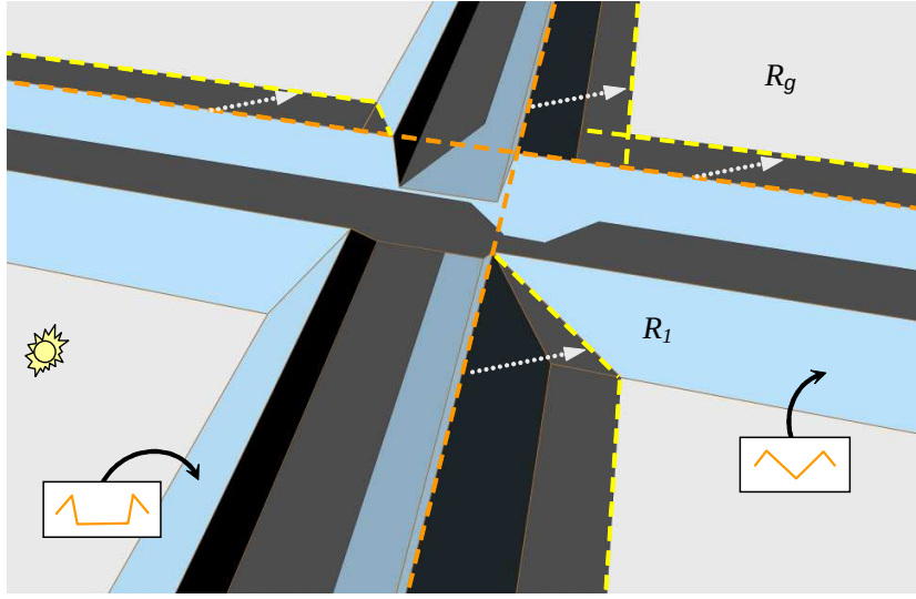
Figure 4.18: Grooves protruding from the surface may produce occlusion to the surrounding surface. The occlusion of the ground facet R_g or the external groove facets, such as R_1 , is computed by only projecting their prolongations (peaks).
