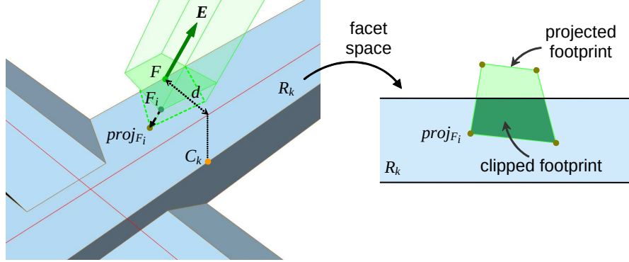
Figure 4.15: Left: footprint is projected onto the current facet following the view direction. Right: once in 2D facet space, the footprint is clipped to the bounds of the facet.
